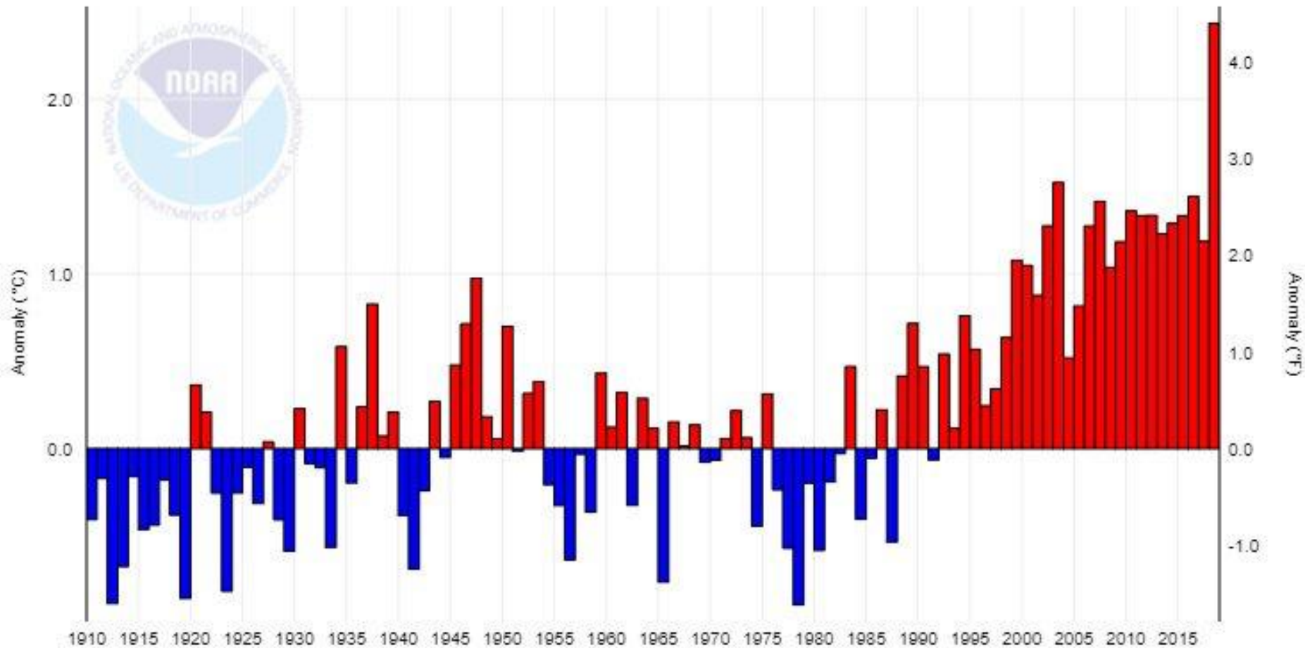
Europe Land Temperature Anomalies, April-August
